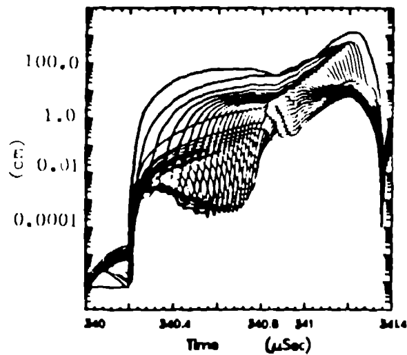
Fig. 6. Radiation mean-free path values for the Lagrangian zones as a function of time. These values are calculated using the Rosseland mean opacities for aluminium from the SESAME tables.
